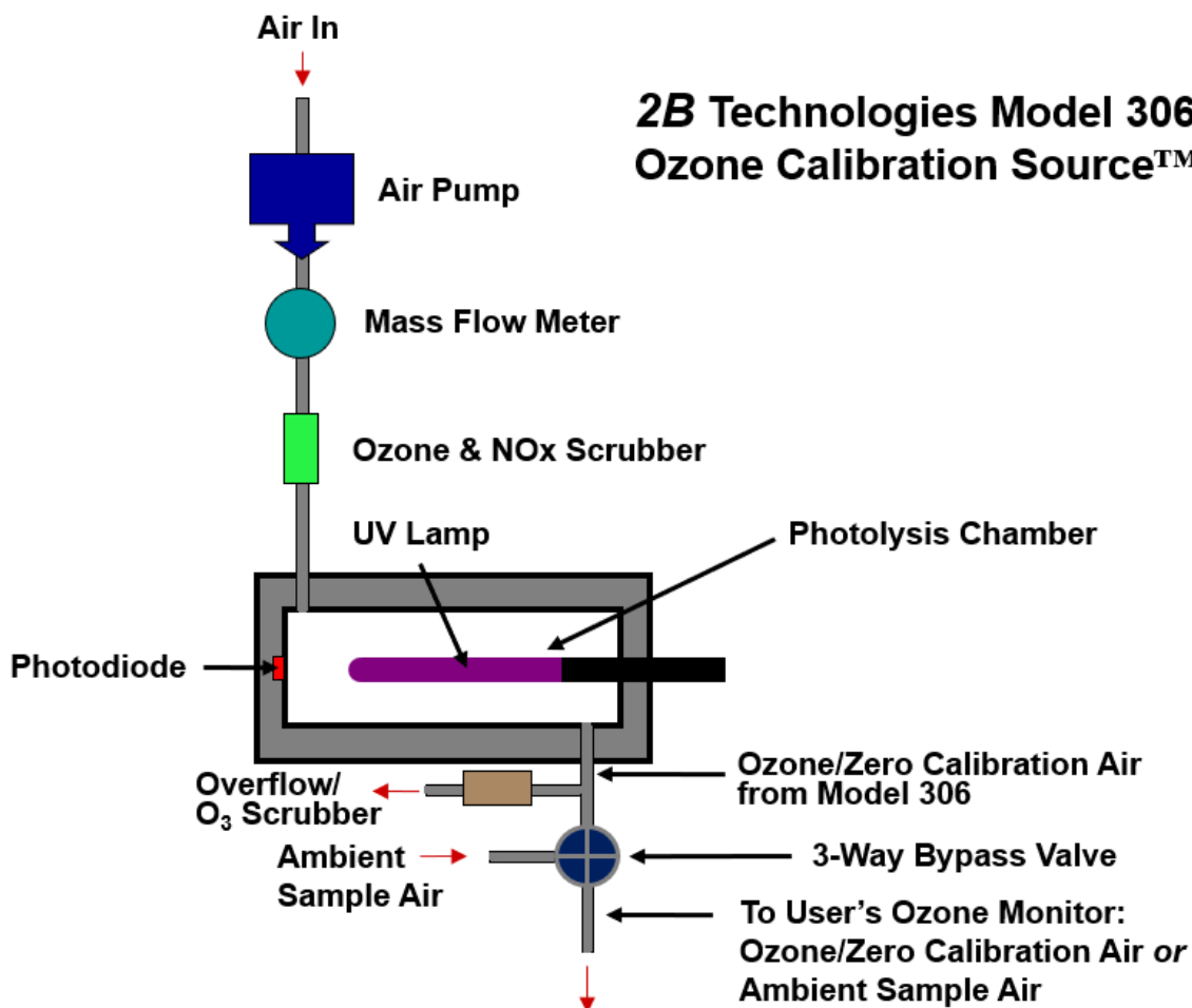
Figure 1-1. Schematic diagram of the Model 306 Ozone Calibration Source™.
