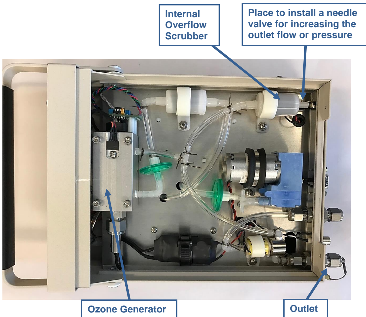
Figure 3-2. Photograph of the Model 306 showing where a needle valve can be installed to increase the flow or pressure at the outlet.
