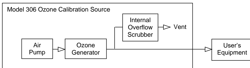
Figure 3-1. Schematic of the Model 306 showing the internal overflow scrubber and vent for any unused portion of the total flow rate.
