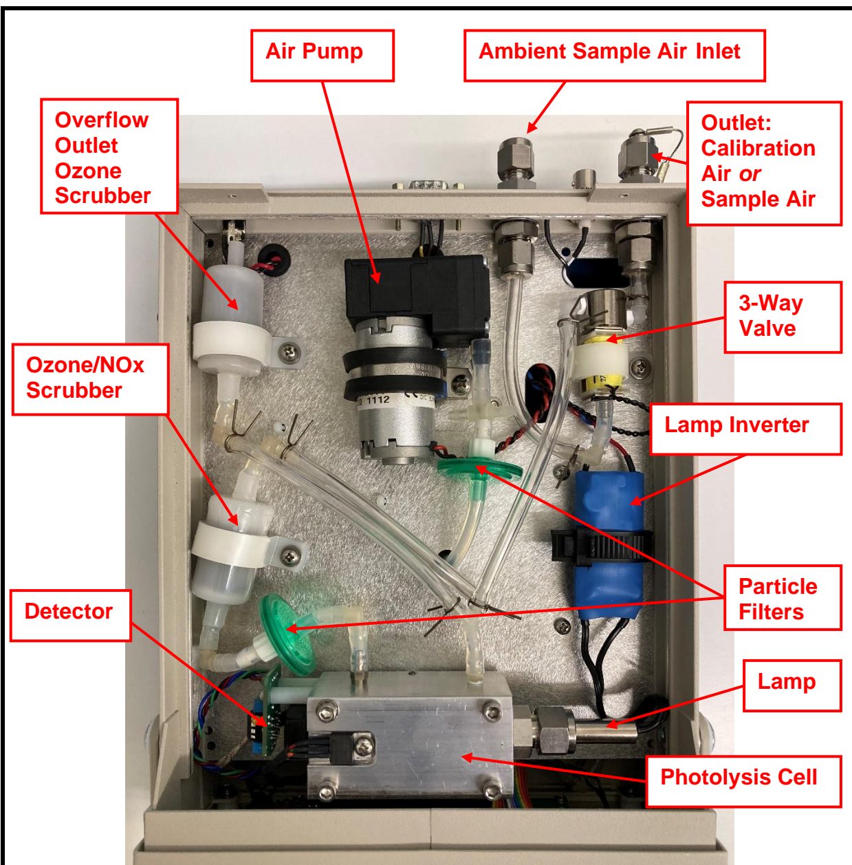
FIGURE 10-1: Bottom view of Ozone Cal Source™ with cover removed. Refer to schematic in Figure 1-1.
