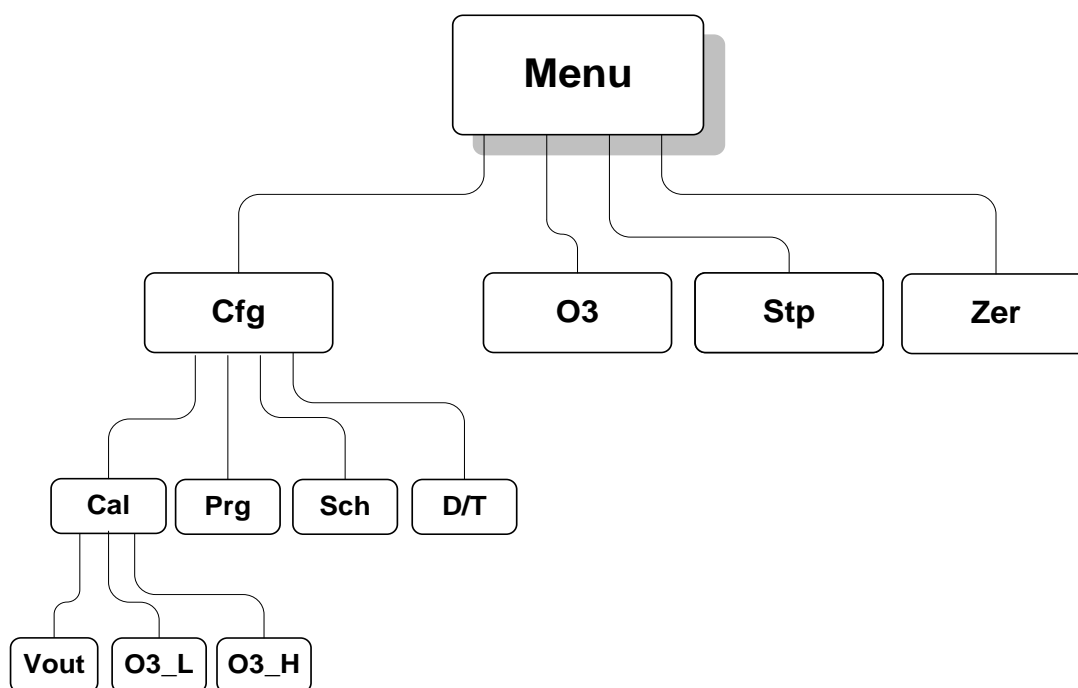
Figure 4-1. The LCD Menu of the Model 306 Ozone Calibration Source™.
