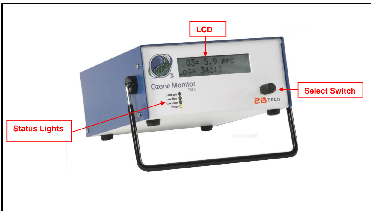
Figure 7.3. Front cover of the Model 106-MFT.
