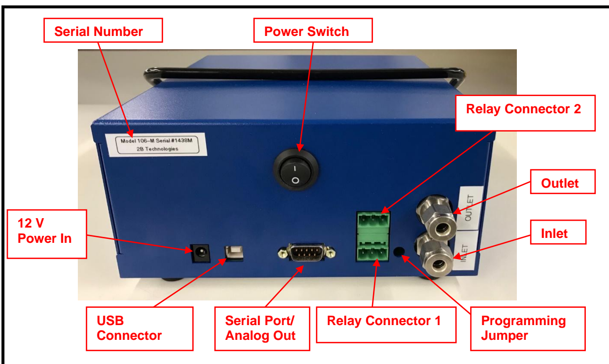
Figure 7.4. Back panel of the Model 106-MFT
