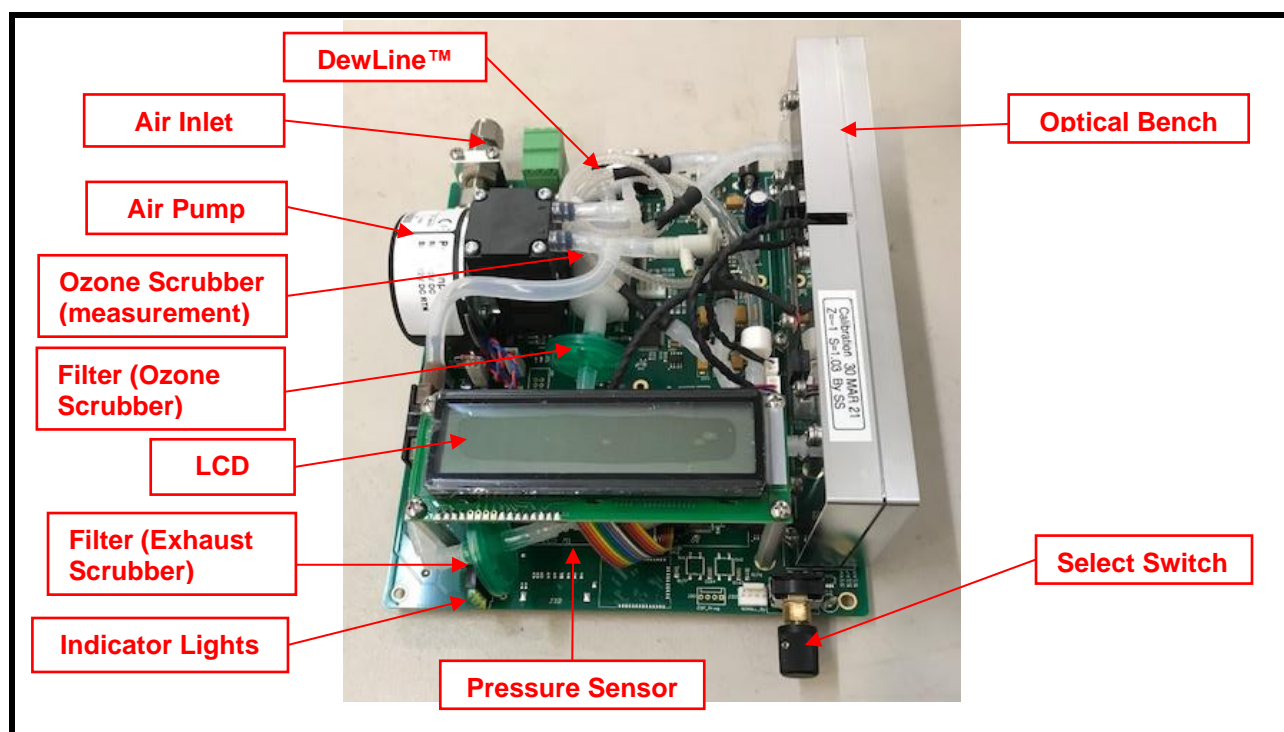
Figure 7.2b. Front view of the OEM-106-L.
