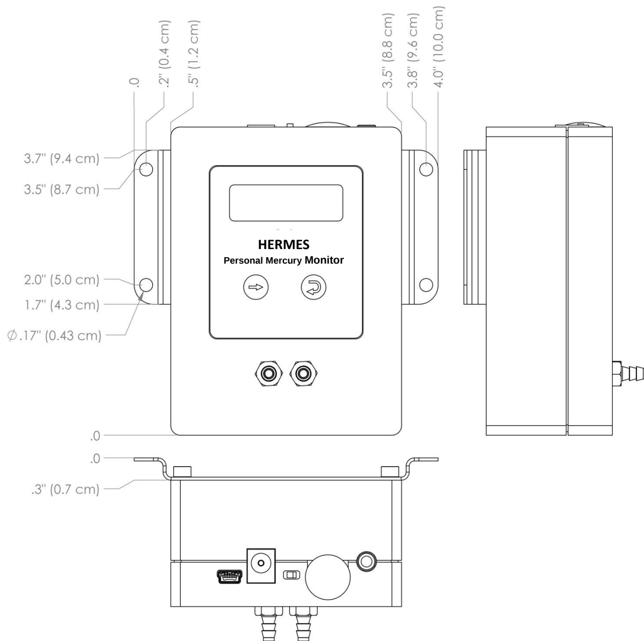
Figure 3. Dimensions of the HERMES with wall mounting bracket.
