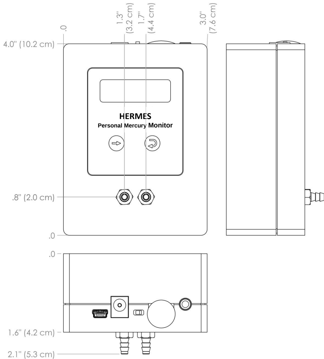
Figure 1. Dimensions of the HERMES.
