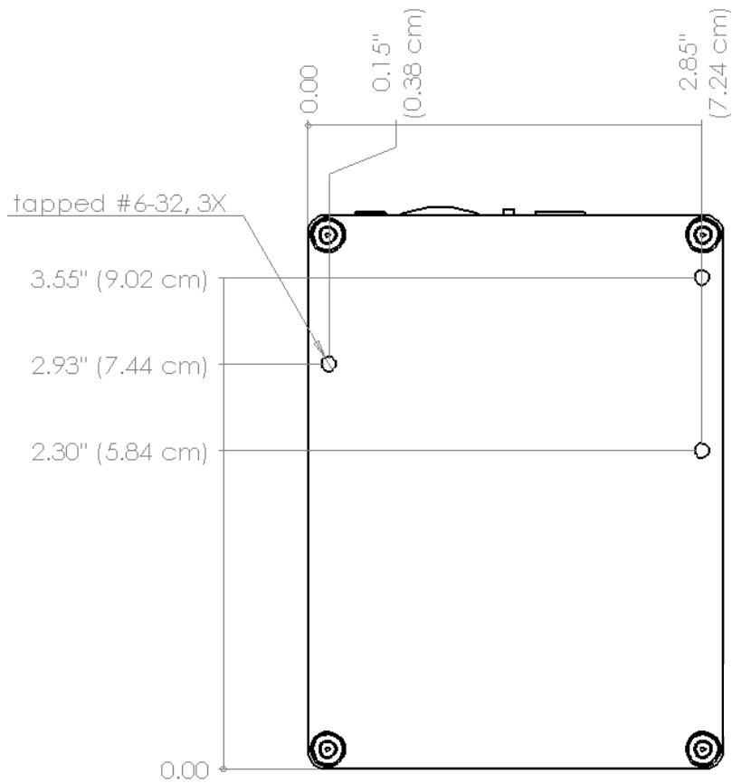
Figure 4. Mounting holes on the back of the Hermes.
