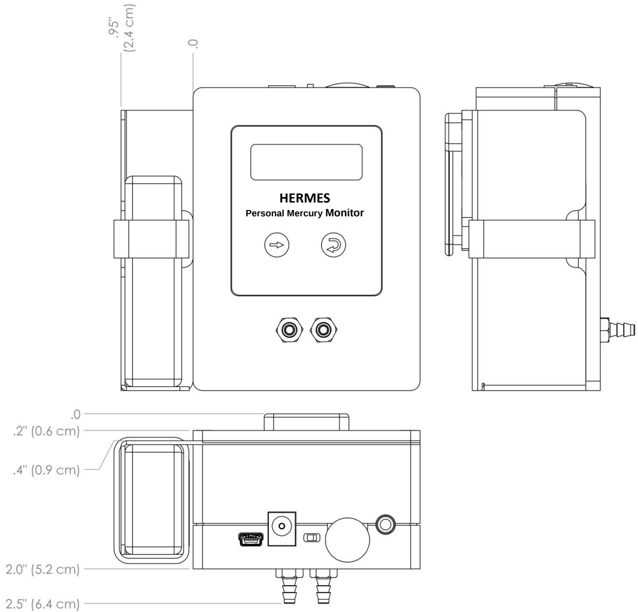
Figure 2. Dimensions of the HERMES with battery bracket and battery.
