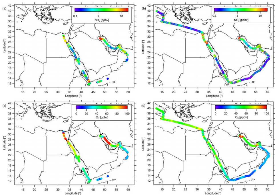
Figure 2. Ship cruises with color-scaled \text{NO}_x mixing ratios during (a) the first and (b) the second leg, and color-scaled \text{O}_3 mixing ratios during (c) the first and (d) the second leg.
